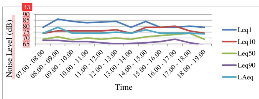
Figure 3. Mandai roundabout noise level chart.
