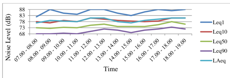
Figure 5. Samata roundabout noise level chart.
